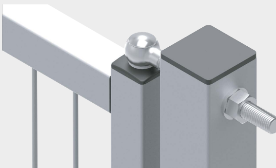
Hinge Hot-dip galvanised LOCINOX hinge with threaded shaft GBM16-DP-40-160 garden
