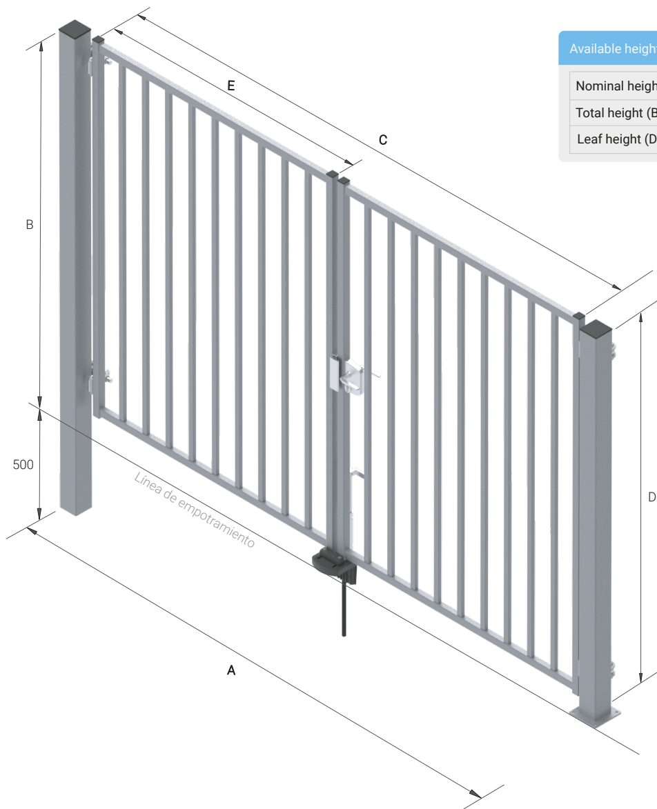
Available widths of the FR14 STYLE and TITAN double leaf gates
