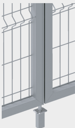
Ground stop seen from the interior Close-up of the IT ground stop
