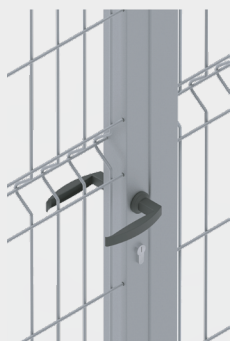
Indusmetal lock seen from the interior Ref. 726 20 mm stainless steel front
