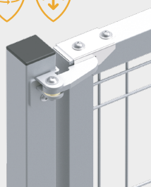
Close-up of the MP50 hinge 180 ° opening and 4-way adjustment
