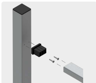
Close-up of the panel fixing system Panel fixing system
